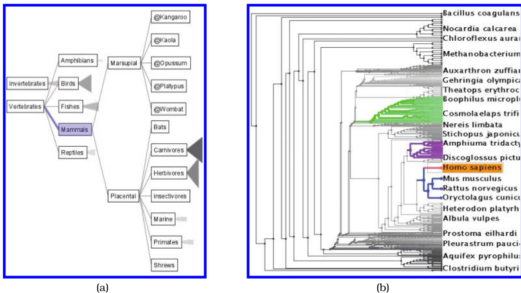
Figure 3.8. Comparing two idioms. (a) SpaceTree [Plaisant et al. 02]. (b) TreeJuxtaposer. From http://www.cs.umd.edu/hcil/spacetreer and [Munzner et al. 03, Figure 1].
