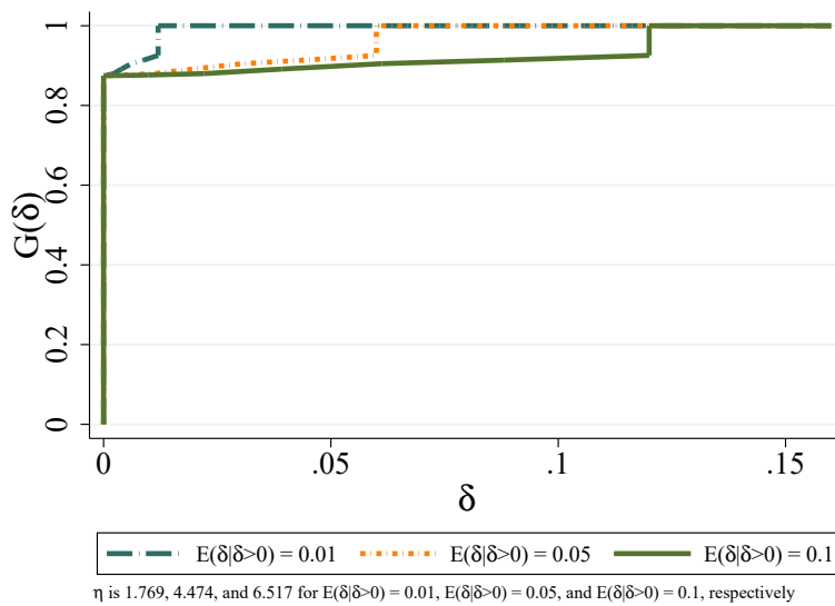
Figure 7: Implied Distribution of \delta Under Constant \eta
