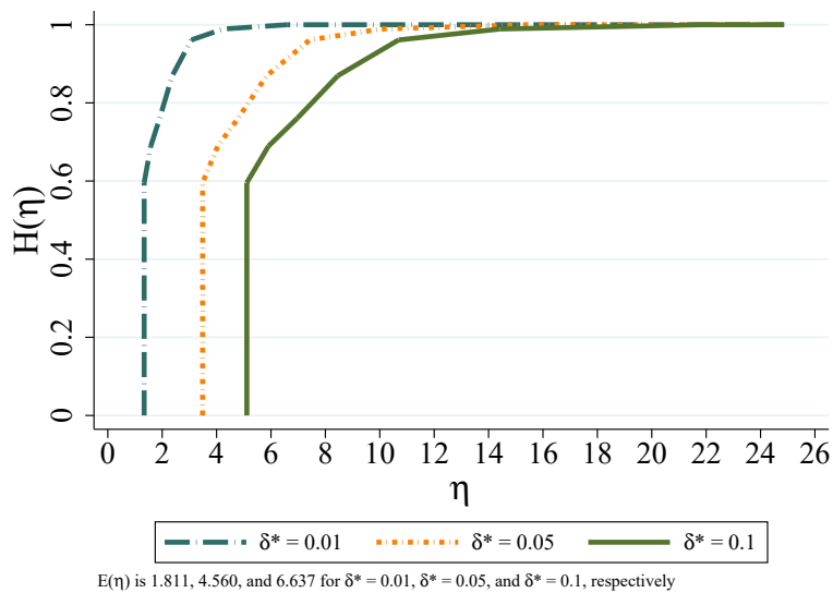
Figure 8: Implied Distribution of \eta with a 2-point Distribution of \delta
