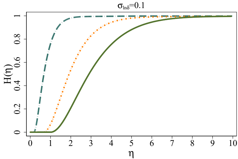
Figure 9: Implied Distribution of \eta using a Deconvolution Estimator where \delta has a Conditional Lognormal Distribution
