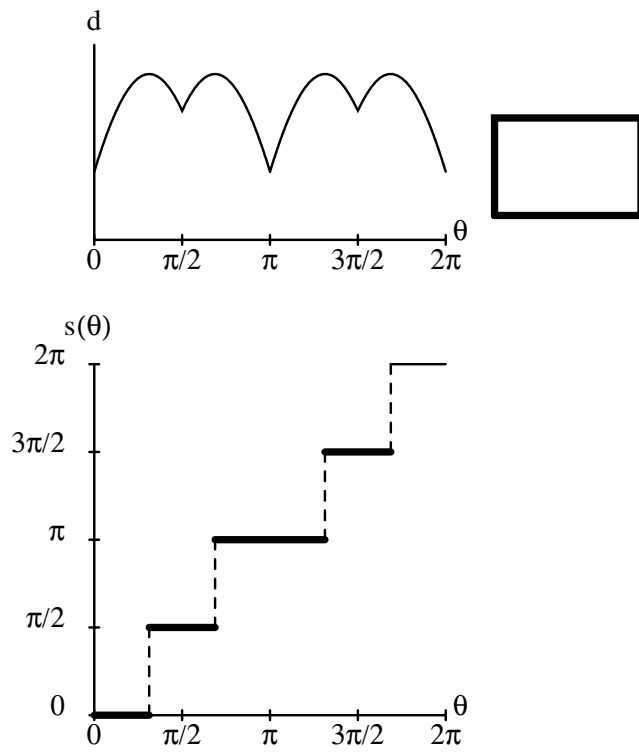
Figure 4: The diameter function (top) and squeeze function (bottom) for the rectangular part.
