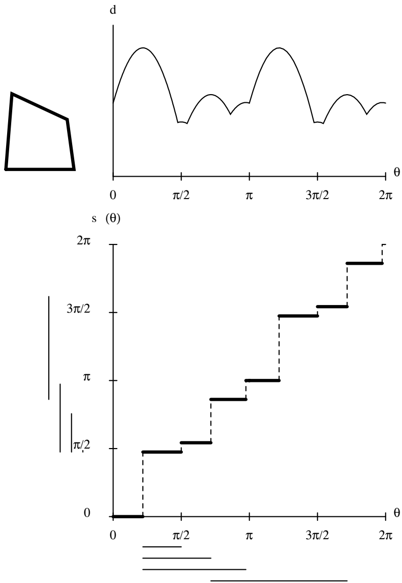
Figure 7: Geometric analysis of the 4gon, showing diameter and squeeze functions. The bars under the horizontal axis indicate the sequence of s -intervals found by the algorithm, the bars to the left of the vertical axis indicate the corresponding s -images .
