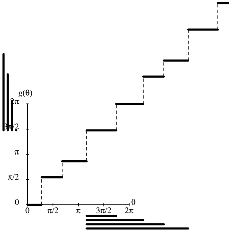
Figure 11: The push-grasp function for the 4gon (unwrapped to show two periods). The bars under the horizontal axis indicate the sequence of s -intervals found by the algorithm, the bars to the left of the vertical axis indicate the corresponding s -images .
