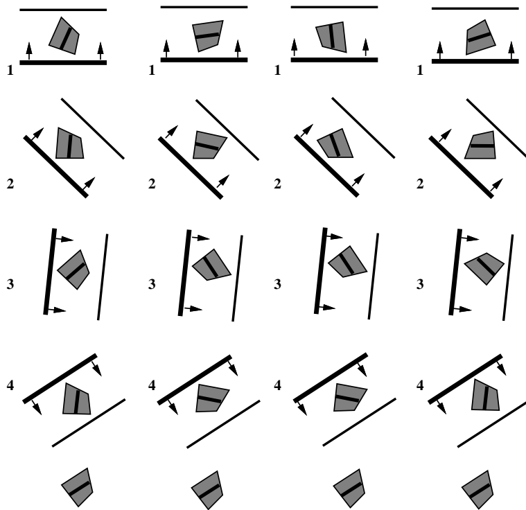
Figure 12: Four traces of push-grasp plan for 4gon, where darkened line indicates pushing jaw. Push-grasp actions are at 0^\circ , -44^\circ , -96^\circ , -146^\circ .
