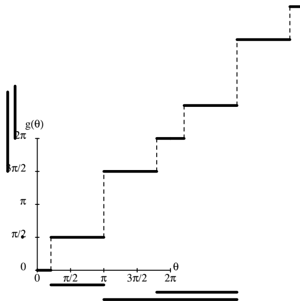
Figure 14: The push-grasp function for the house-shaped part (unwrapped to show two periods). The bars under the horizontal axis indicate the sequence of s -intervals found by the algorithm, the bars to the left of the vertical axis indicate the corresponding s -images .
