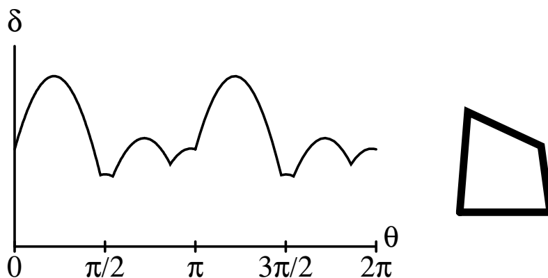
Figure 16: The diameter function for the four-sided part shown at the right in its zero orientation. During a squeeze, the part rotates so as to reduce the diameter, terminating when the diameter reaches a local minimum.
