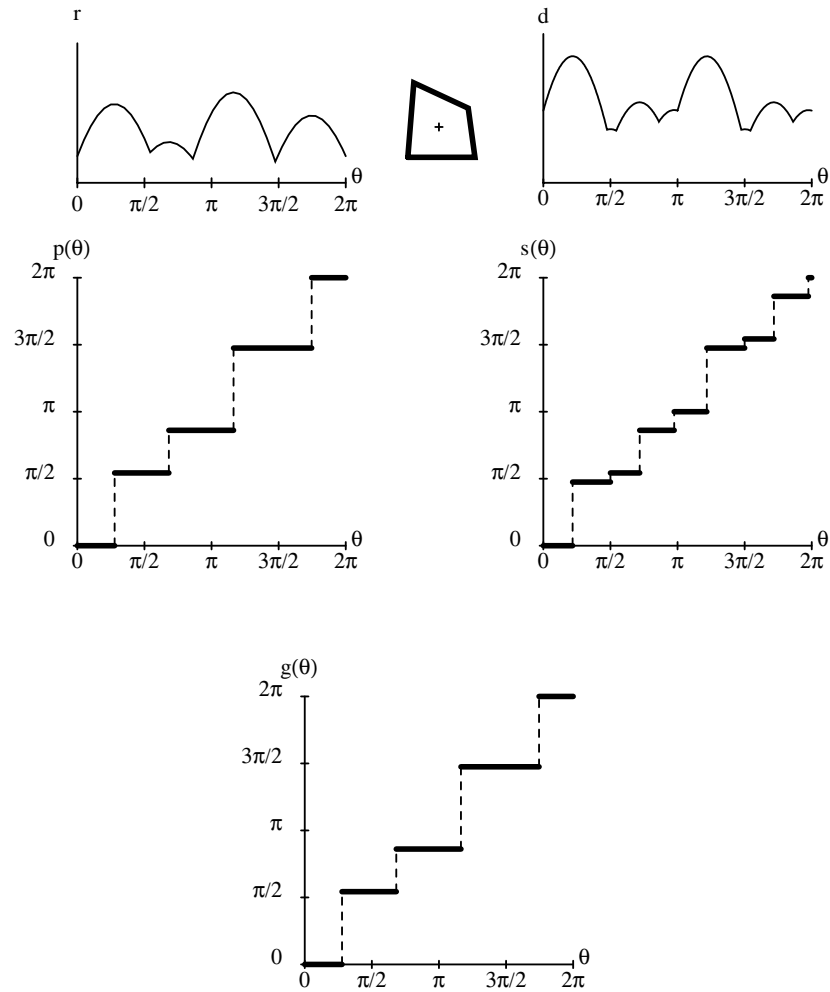
Figure 10: Push-grasp analysis for the four-sided part. In the upper left is the radius function. Directly below it is the push function. In the upper right is the diameter function. Directly below it is the squeeze function. The push-grasp function is shown at the bottom.
