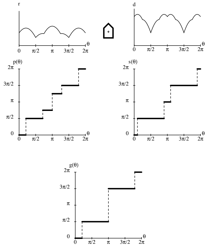
Figure 13: Push-grasp analysis for the house-shaped part. In the upper left is the radius function. Directly below it is the push function. In the upper right is the diameter function. Directly below it is the squeeze function. The push-grasp function is shown at the bottom.
