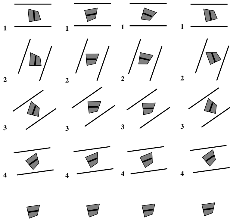
Figure 8: Four traces of the resulting squeeze plan for the 4gon.
