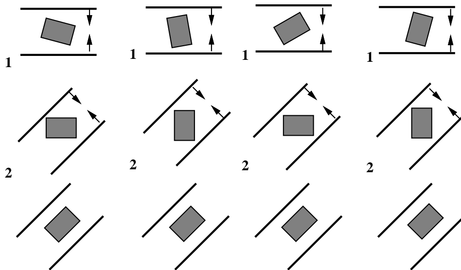
Figure 3: Four traces, running from top to bottom, of a two-stage plan for orienting a rectangular part. Each squeeze action is indicated with a pair of bold parallel lines. In the absence of friction between the part and the jaws, the part will always rotate into a vertical or horizontal orientation after the first action at 0^\circ . After the second action at 45^\circ , the part is constrained to be in one of two symmetric orientations.
